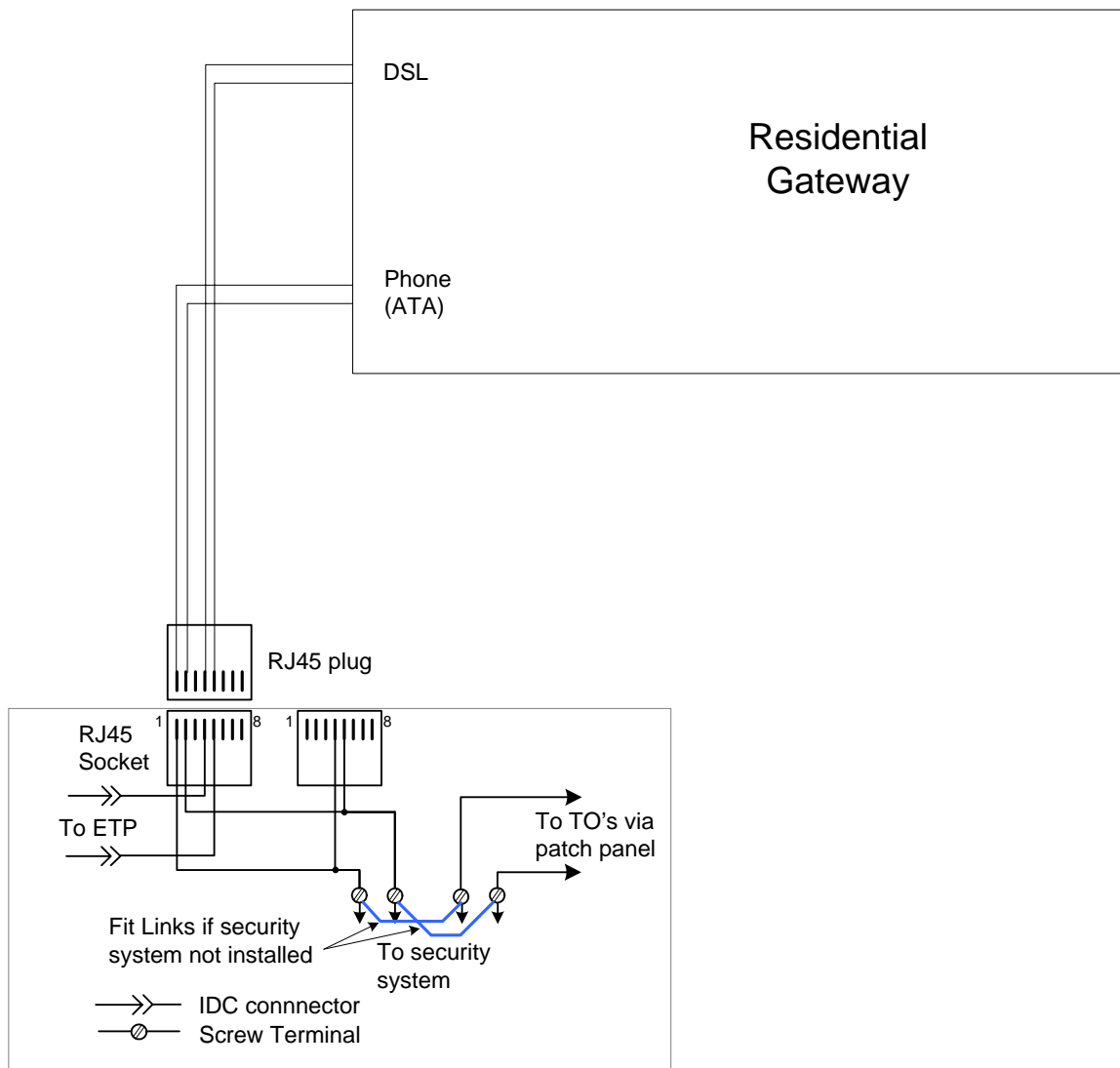
Connection of a Residential Gateway to a DTP using single cable
