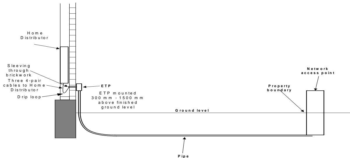
TYPICAL LEAD-IN ARRANGEMENT AND CONNECTION TO HOME DISTRIBUTOR
