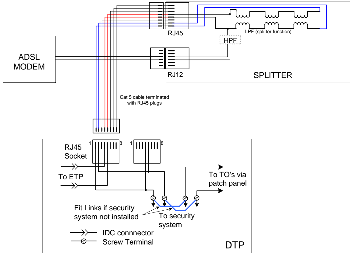
Connection of DSL Splitter at DTP using single cable
