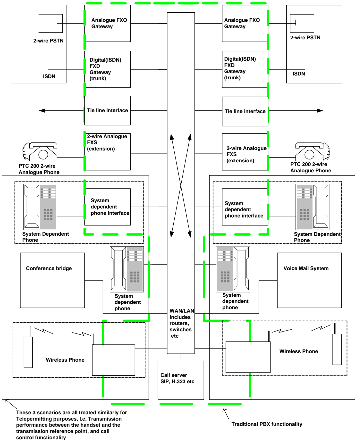
Fig 3.1 Elements of a private voice network
